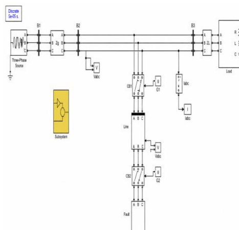
Fig3: simulation model
