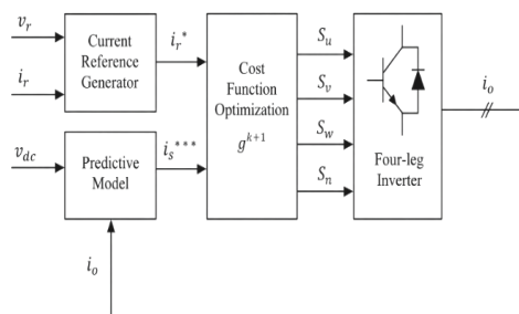
Fig2. Proposed predictive digital current control block diagram.
