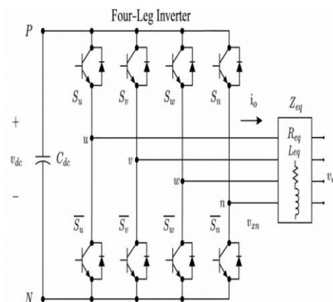
Fig1. Two-level four-leg PWM-VSI topology.
